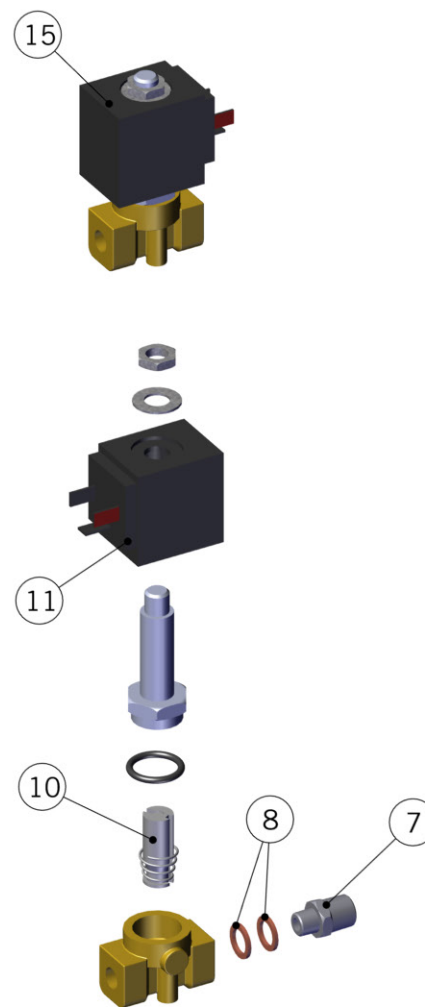
3-WAY SOLENOID VALVE HOT WATER
